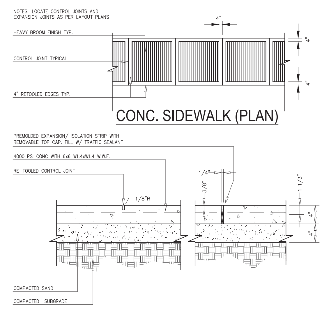
4" CONCRETE PAVEMENT
