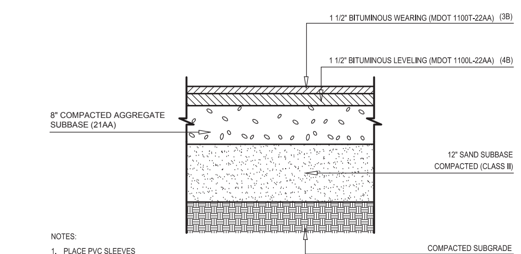
ASPHALT PAVEMENT SECTION
