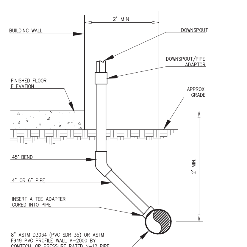
ROOF DRAIN CONNECTION DETAIL
